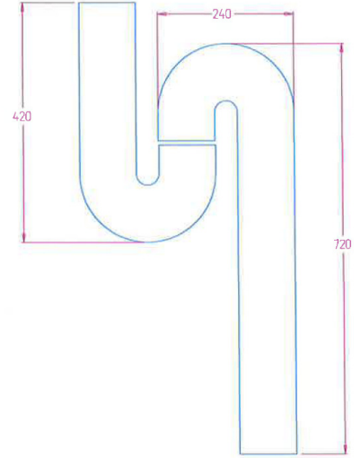
100mm "S" trap
